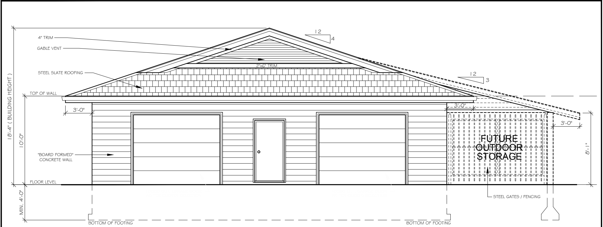
FRONT ELEVATION
